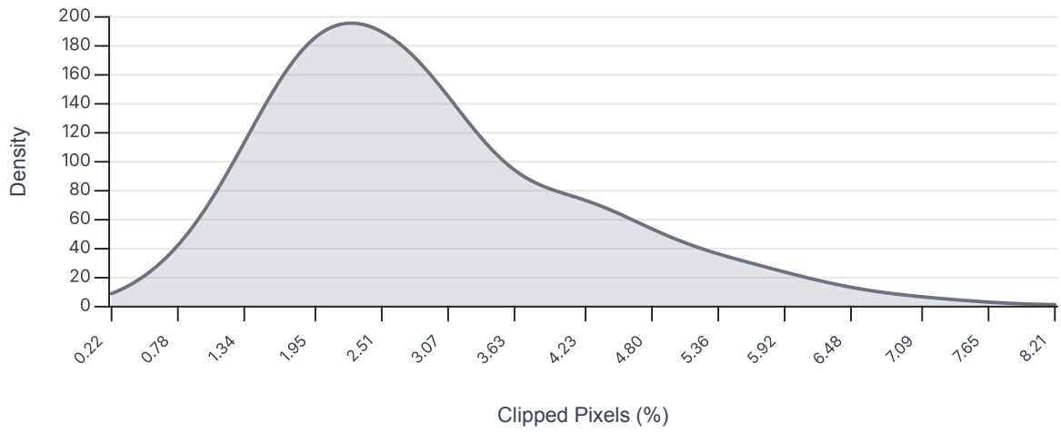
Clipped Pixels
