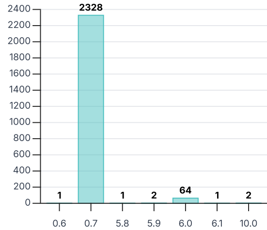
Bitrate (Mbps)
