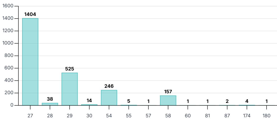
Min GOP
